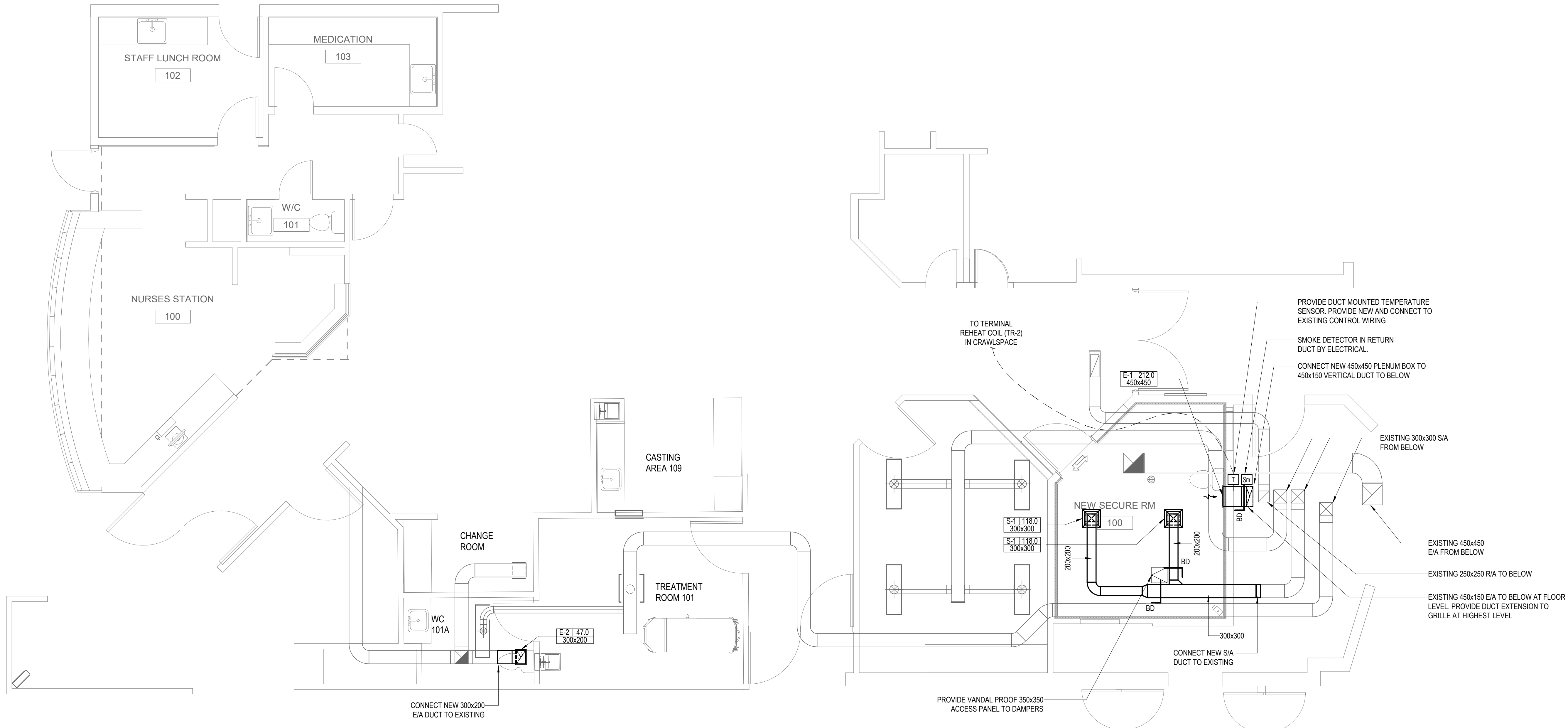
1 MAIN FLOOR HVAC NEW CONSTRUCTION PLAN 1 : 50
