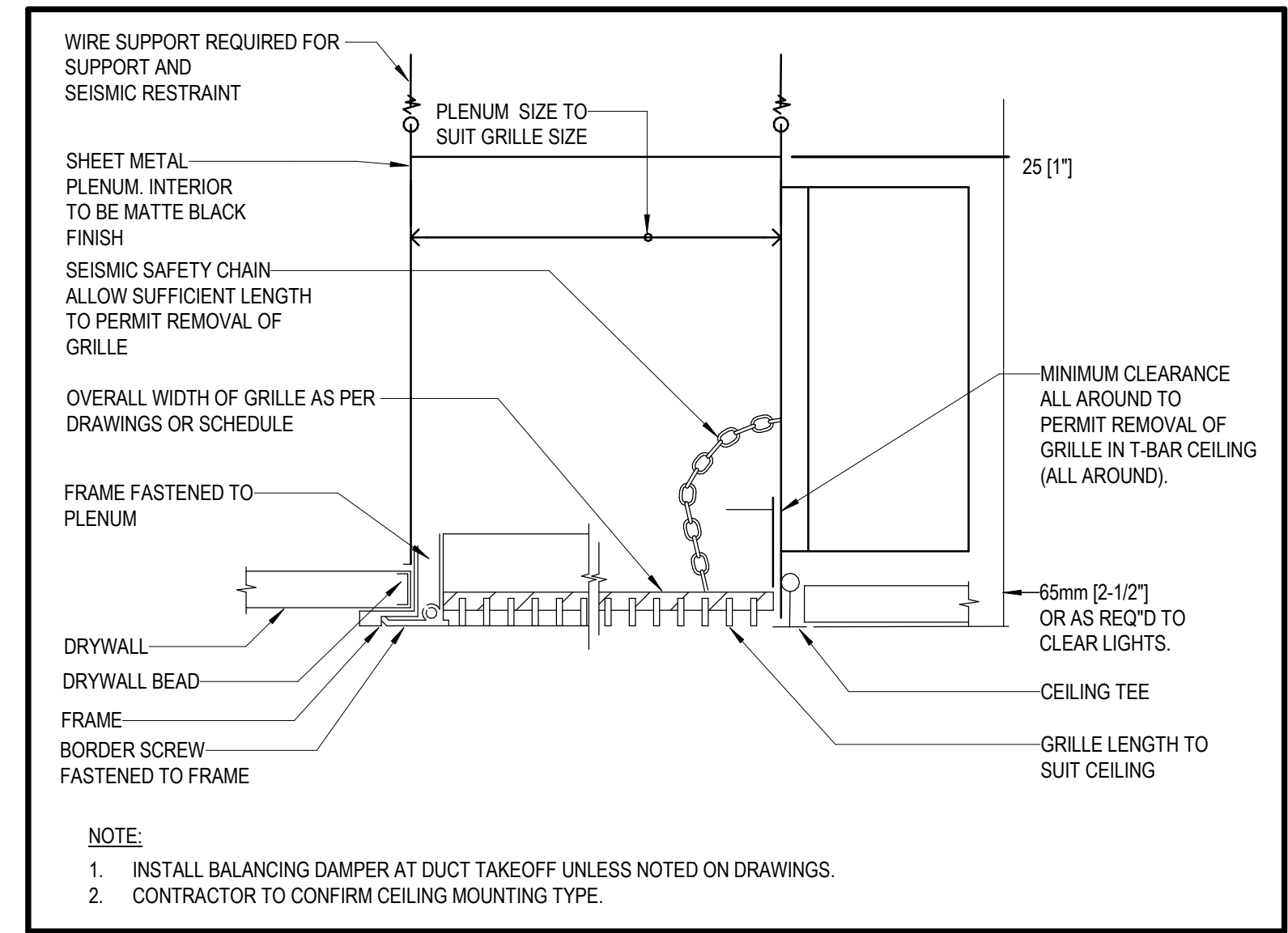
3 WASHROOM EXHAUST GRILLE NTS
