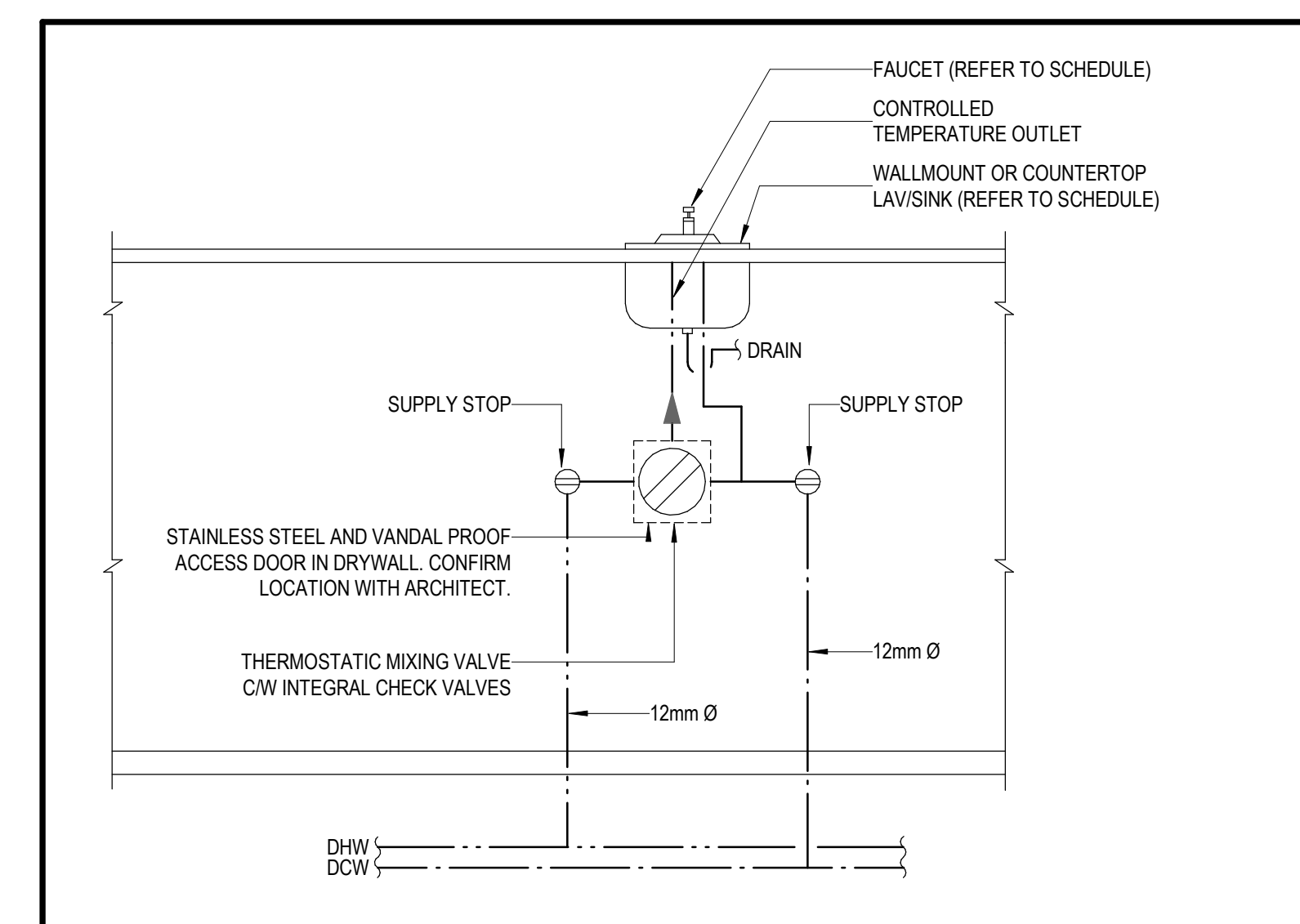
2 LAVATORY/SINK THERMOSTATIC MIXING VALVE PIPING DIAGRAM NTS
