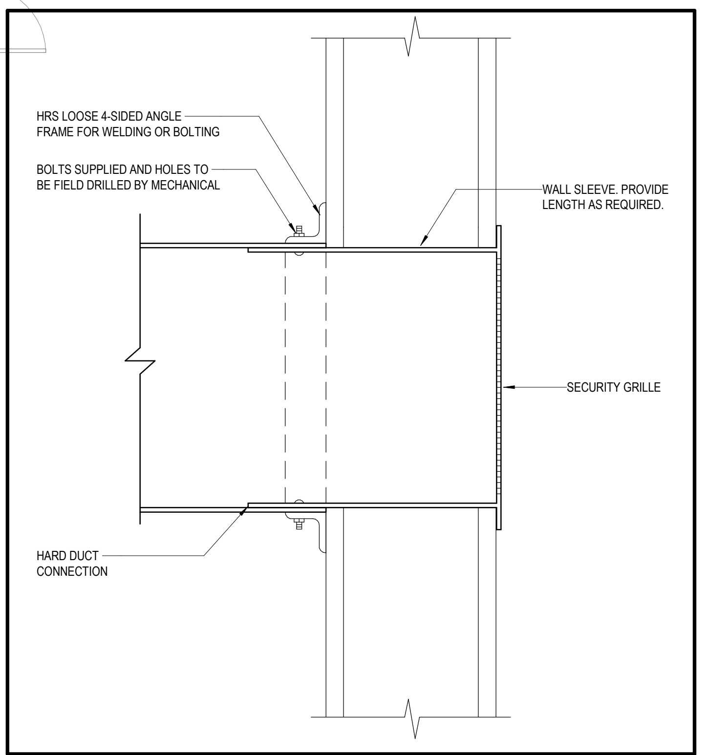
4 SIDEWALL MOUNTED SECURITY GRILLE NTS
