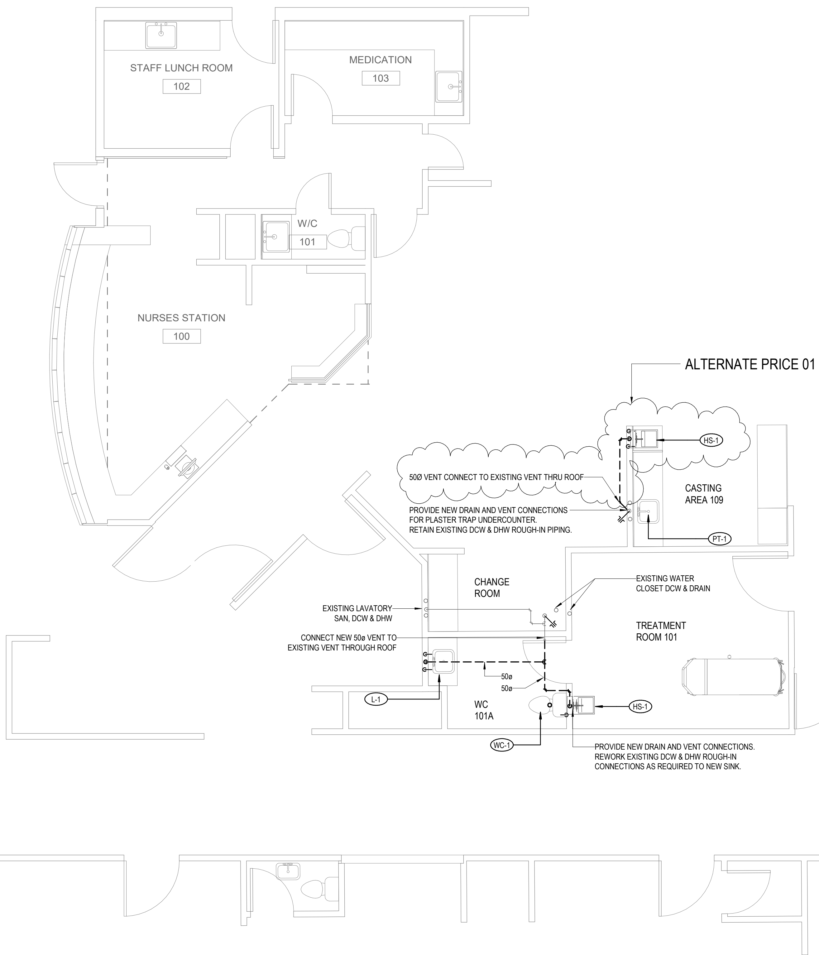
1 MAIN FLOOR PLUMBING & FIRE PROTECTION NEW CONSTRUCTION PLAN 1 : 50
