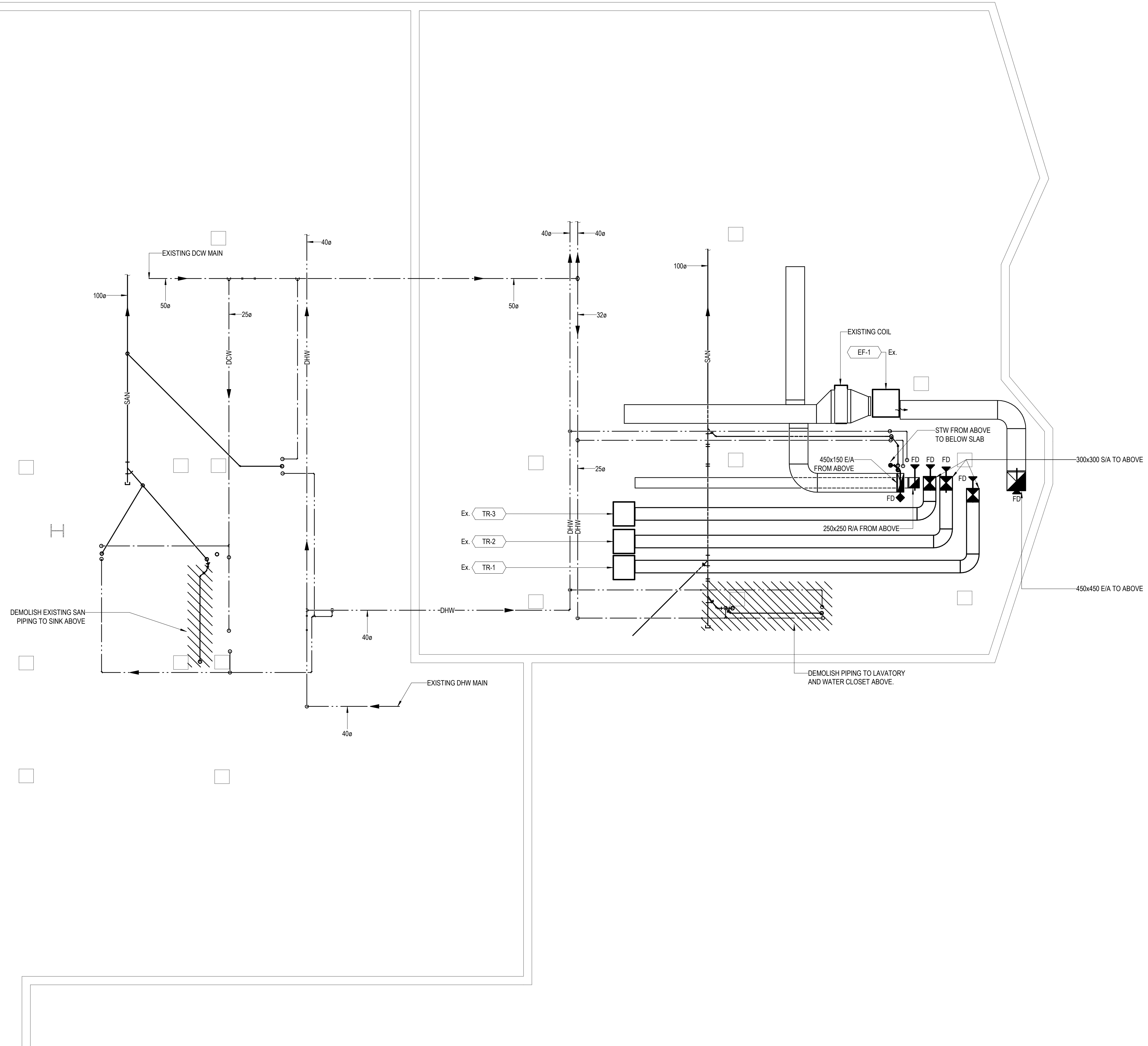
1 CRAWLSPACE MECHANICAL DEMO PLAN 1:50
