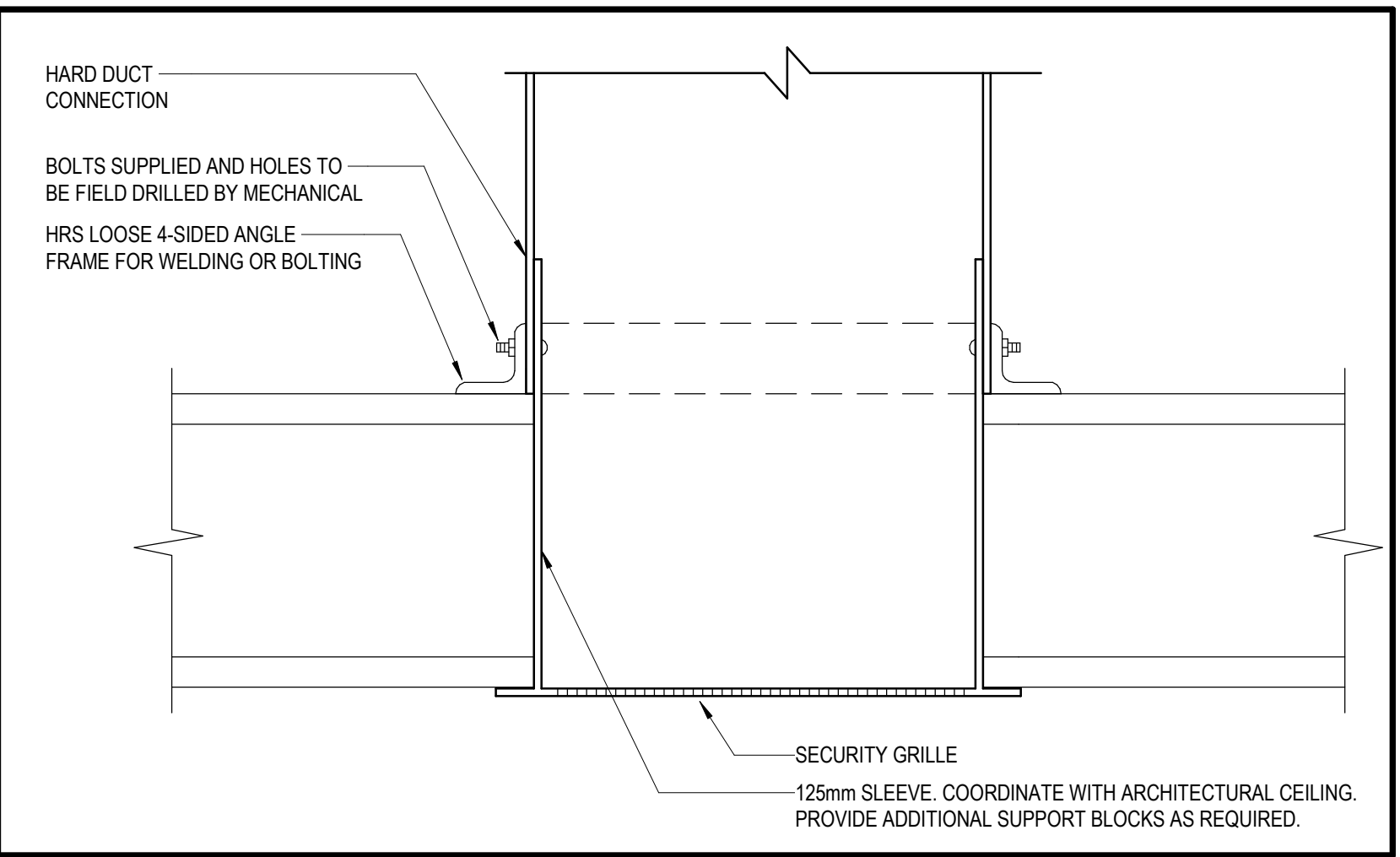
2 CEILING MOUNTED SECURITY GRILLE NTS
