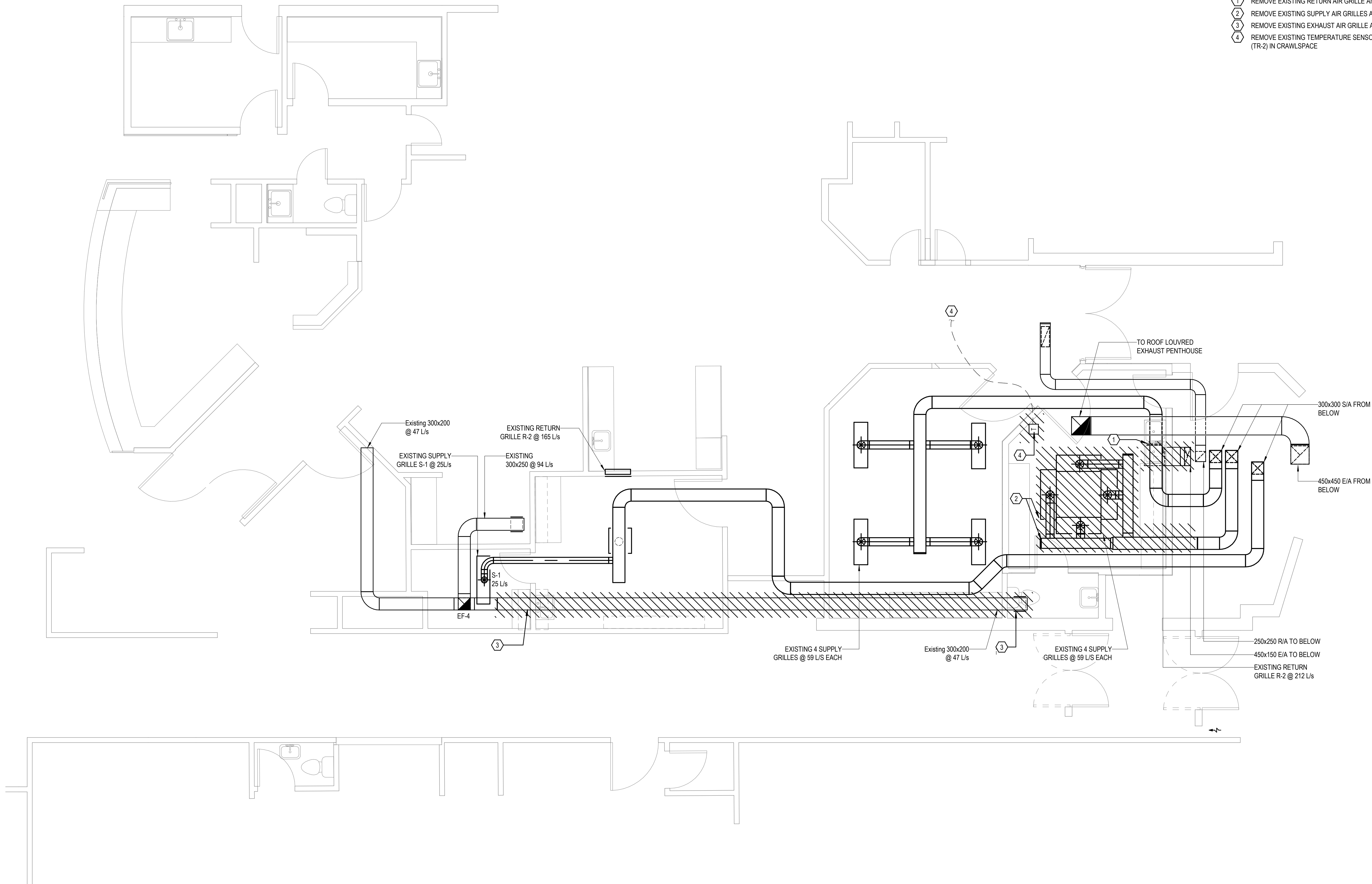
1 MAIN FLOOR HVAC DEMO PLAN 1 : 50
