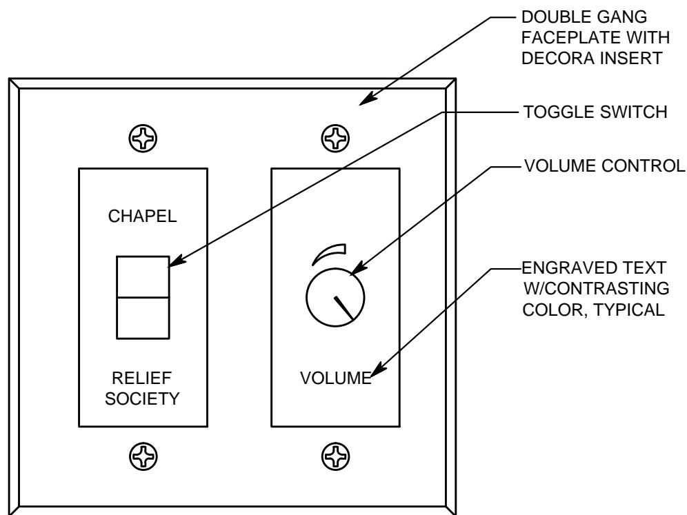
4 MOTHERS ROOM CONTROLLER NO SCALE
