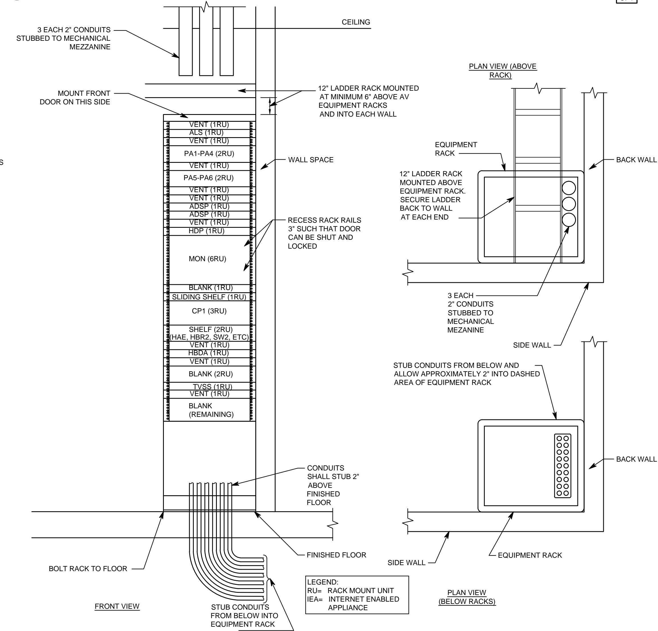
1 EQUIPMENT RACK ELEVATION AND DETAILS NO SCALE
