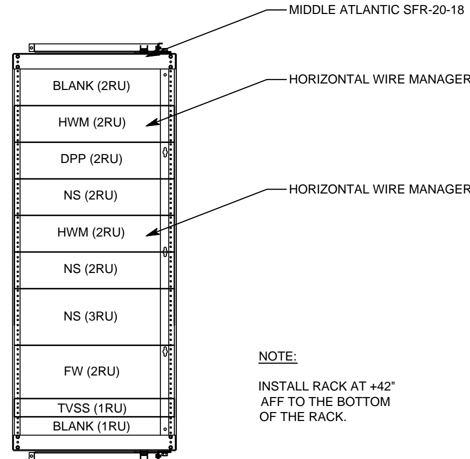
7 DATA RACK ELEVATION NO SCALE
