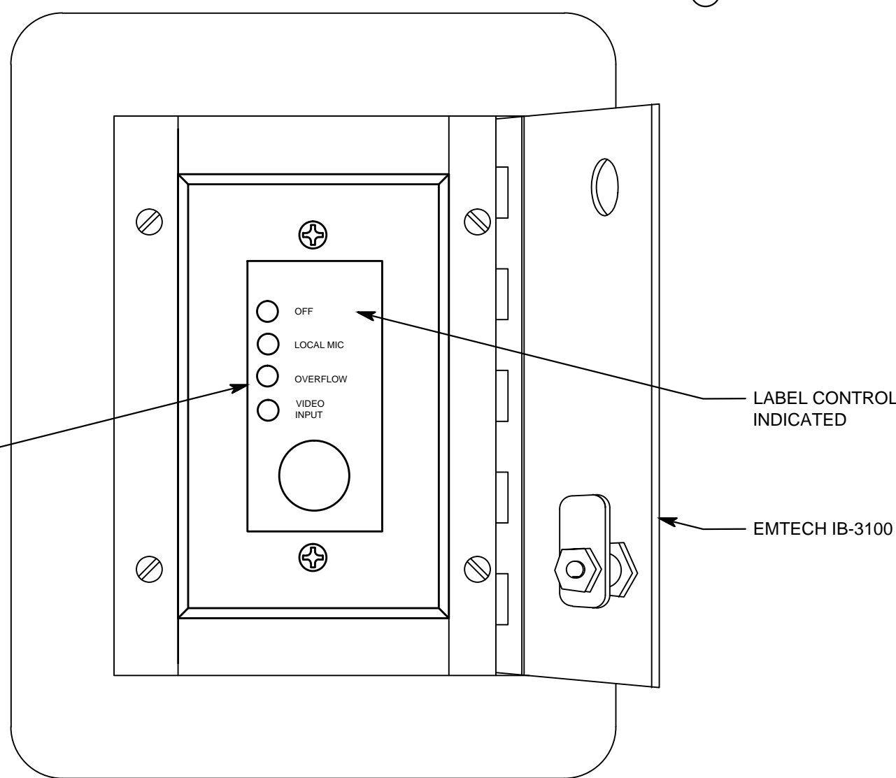
6 MEDIA PANEL (VM) NO SCALE
