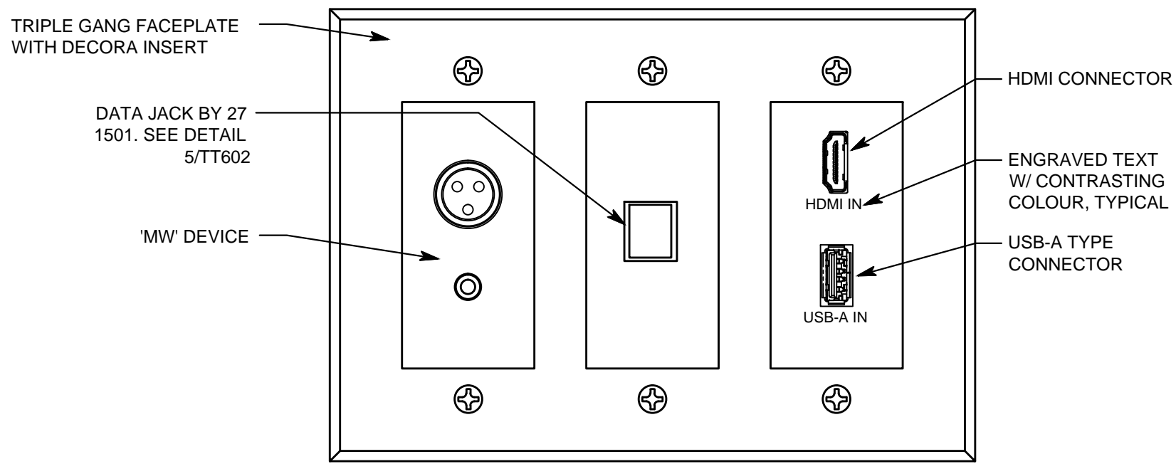
7 CONNECTION PANEL #2 NO SCALE
