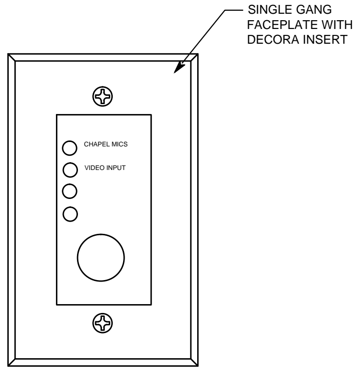
6 MEDIA PANEL (VM) NO SCALE
