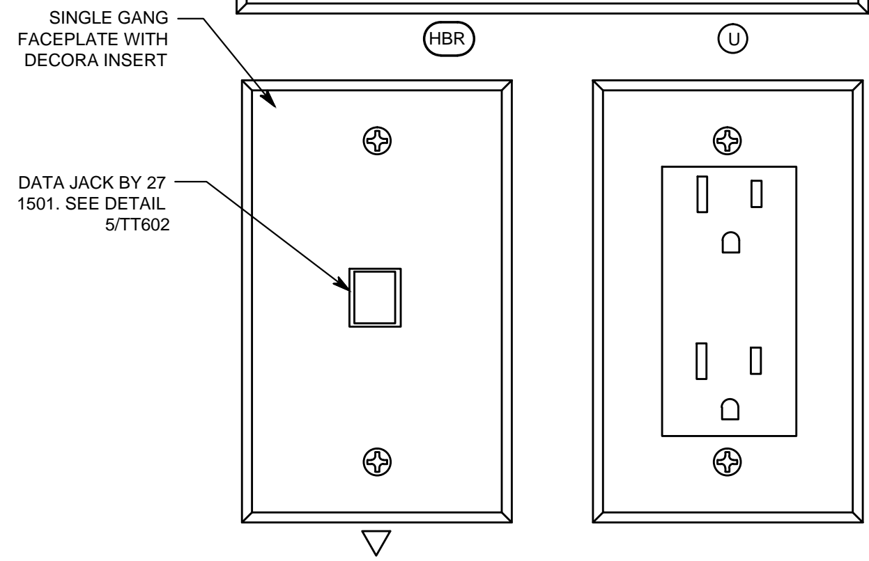
9 PULPIT CONNECTION DETAILS NO SCALE
