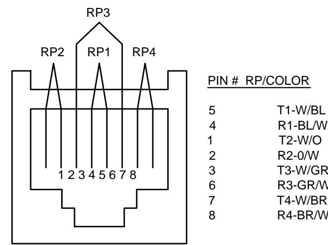
3 OUTLET PINNING DETAIL NO SCALE
