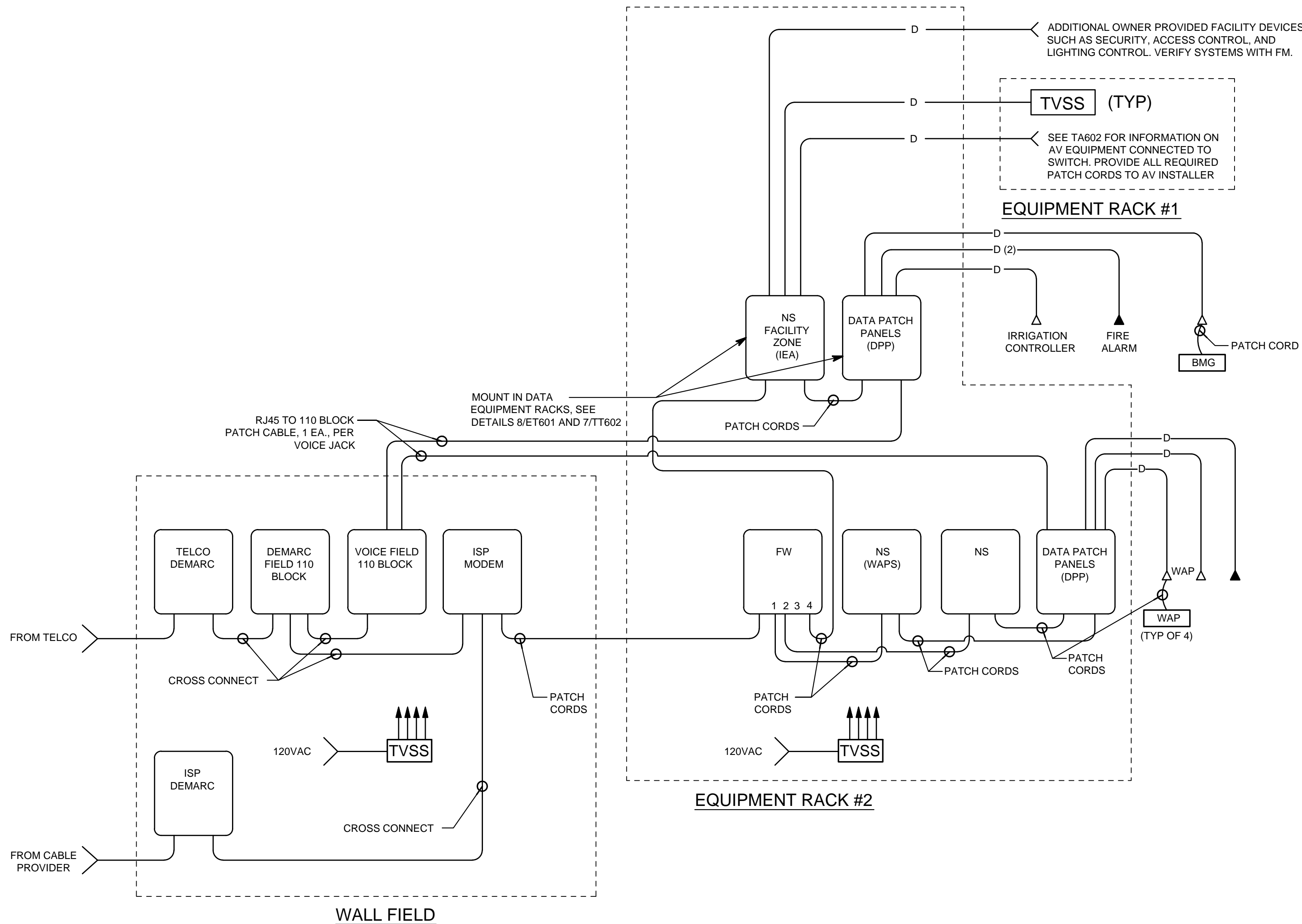
4 STRUCTURED CABLING RISER DIAGRAM
