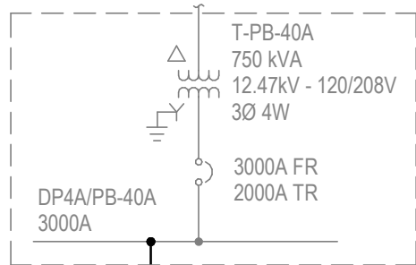
ELECTRICAL ROOM #1 AND #2
